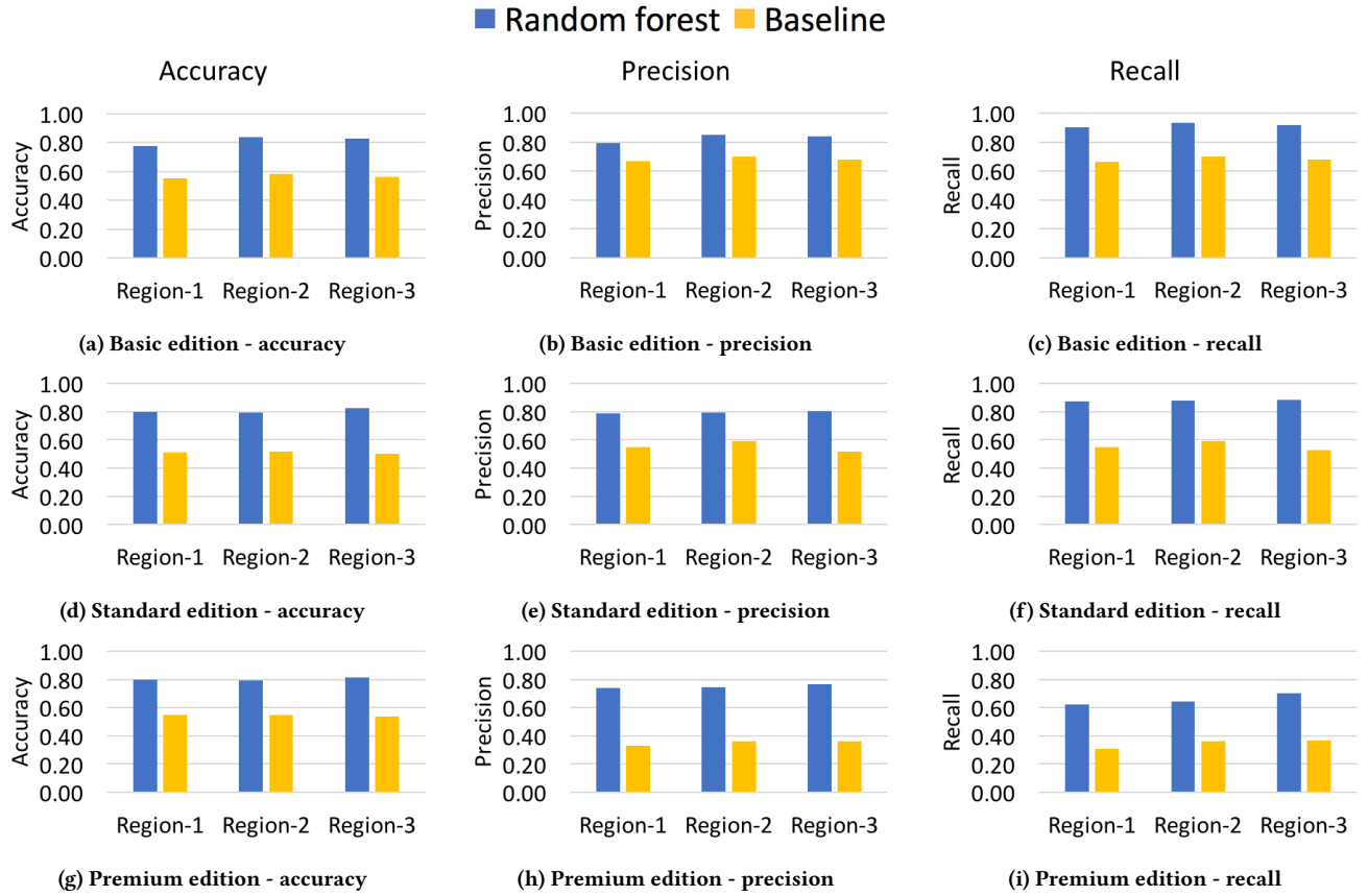
Figure 5: Results of predicting database lifespan over Basic (top), Standard (middle), and Premium (bottom) editions for the whole population.
